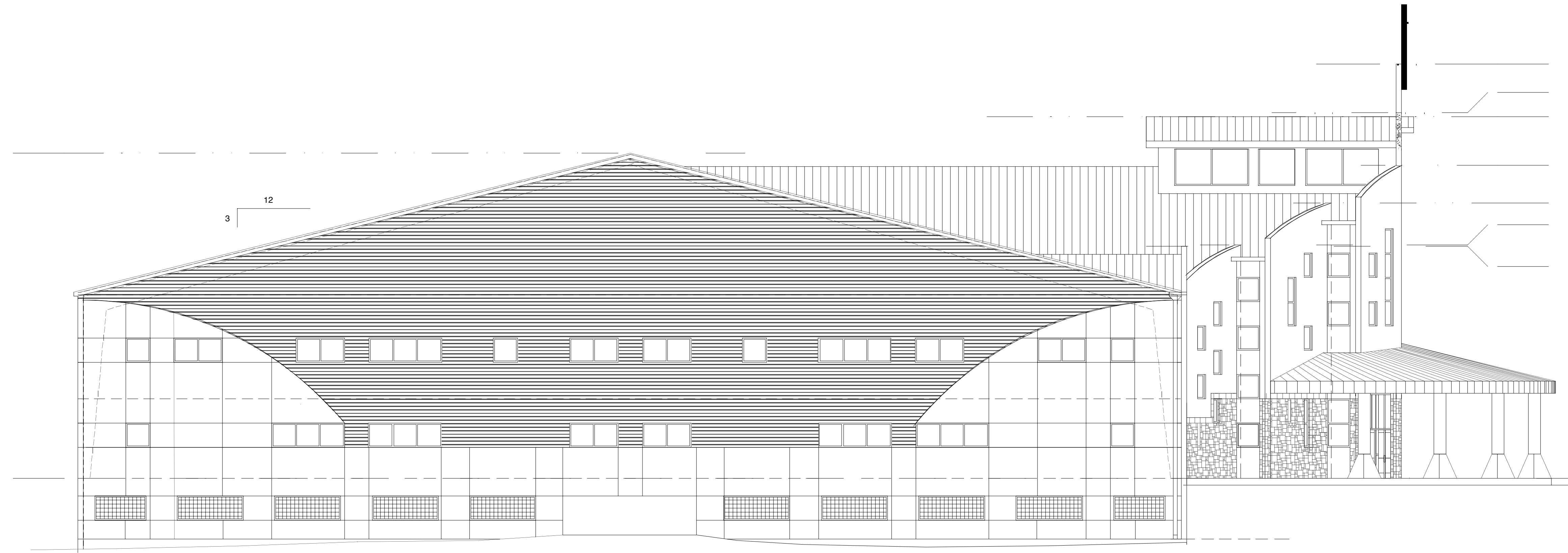
1 LEFT (WEST) SIDE ELEVATION 3/32" = 1'-0"
