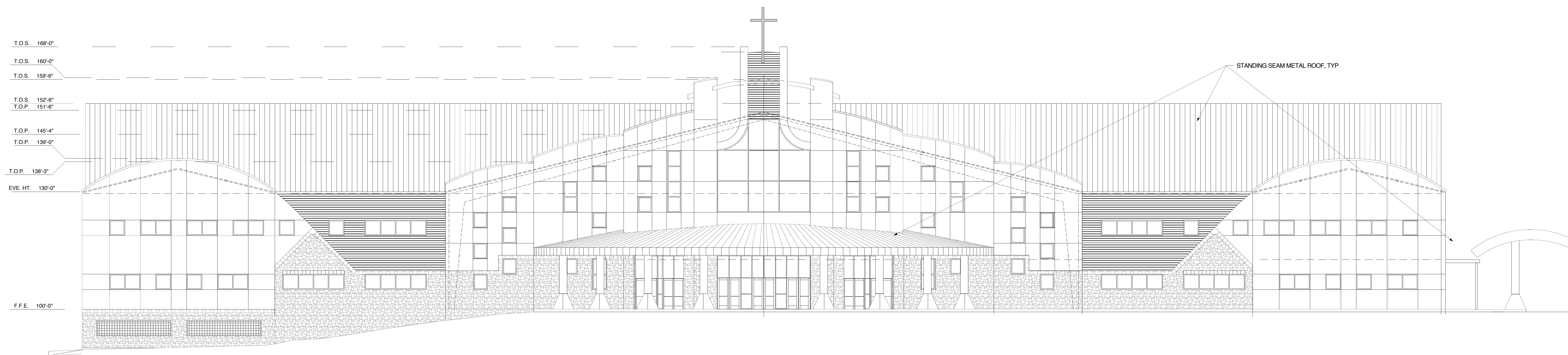
2 RIGHT (EAST) SIDE ELEVATION 3/32" = 1'-0"
