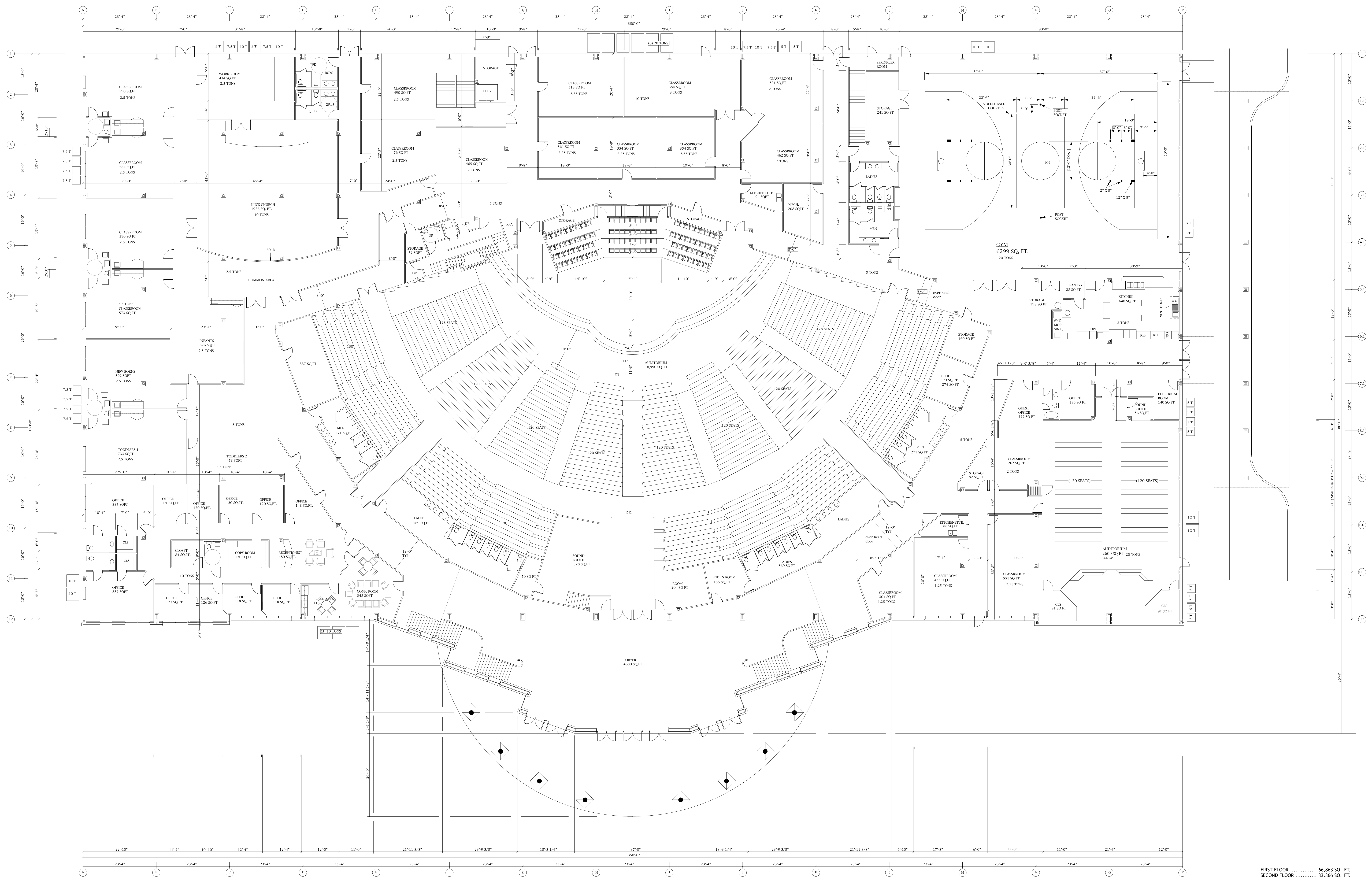
FLOOR PLAN 3/32" = 1'-0"
